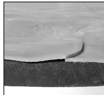
XLPE with Linear Liner Actual sodium hypochlorite tank; shows thin liner, delamination, cracking, etc.
