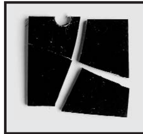
XLPE exposed 6 months in 98% H 2 SO 4 3.4 ft. pounds @ -40° F.
